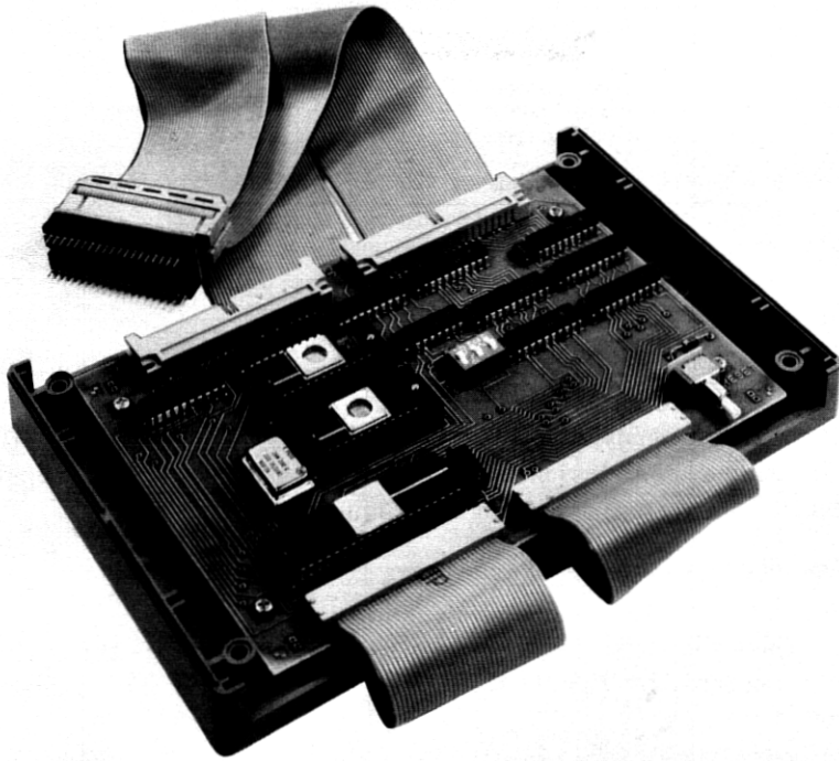
Fig. 6—Digital signal processor EMULATOR prototyping board.
